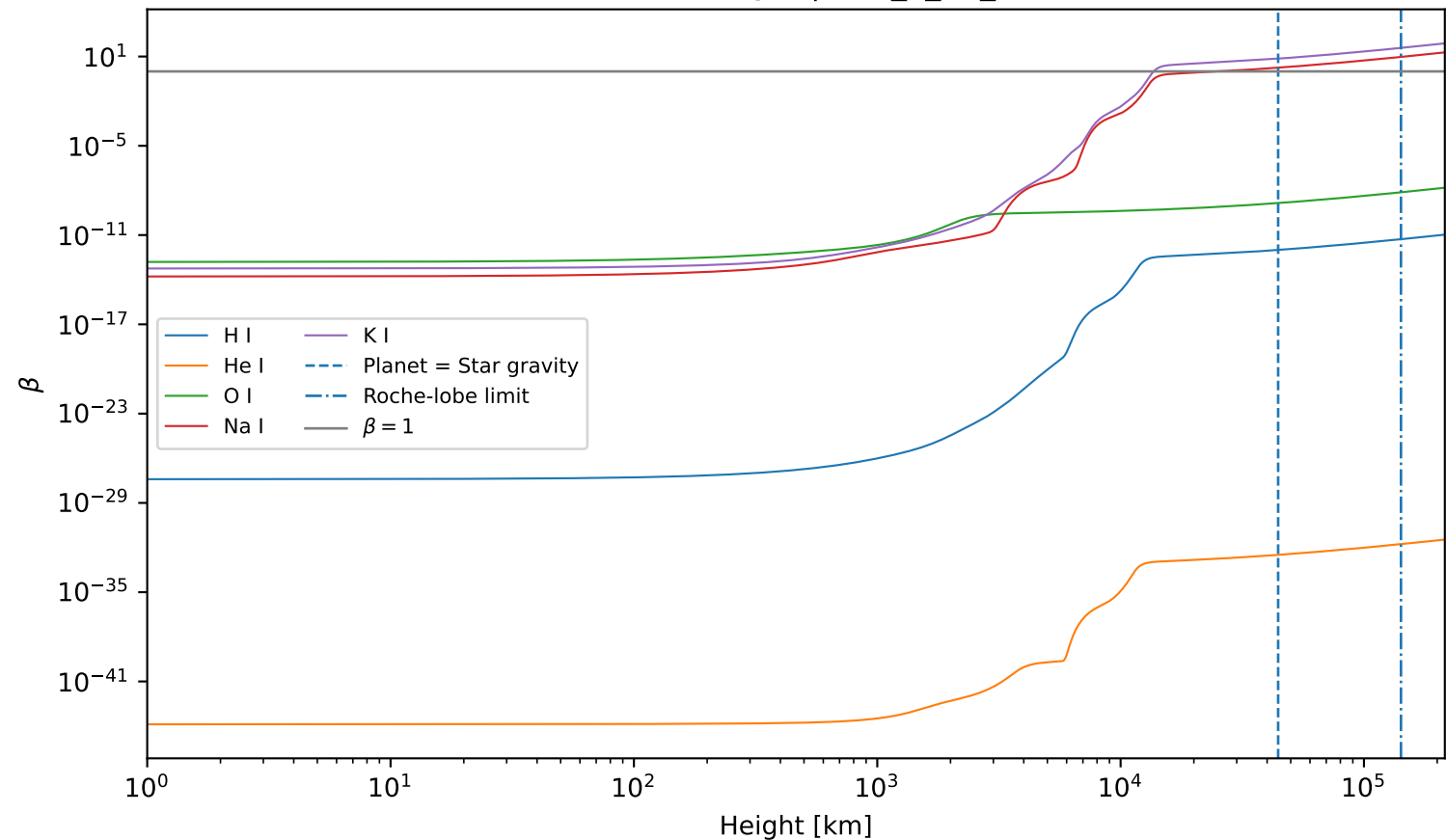
Beta vs height | HAT_P_11_b
